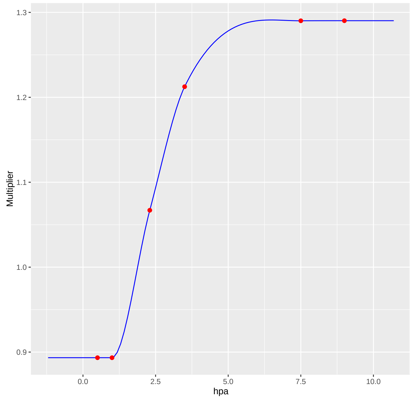
Spline Shape For: hpa
